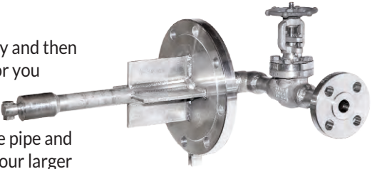
WTZ Lance with Inlet Valve and Gussets
