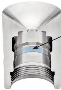
Cutaway view of carrier showing BETE's unique locking lug feature
